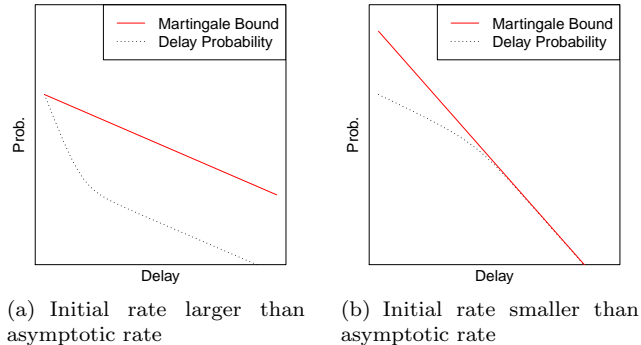
Figure 6: Possible CCDF of the delay. Depending on the flows’ burstiness the martingale (exponential) bounds are inevitably loose for small or large delays.
