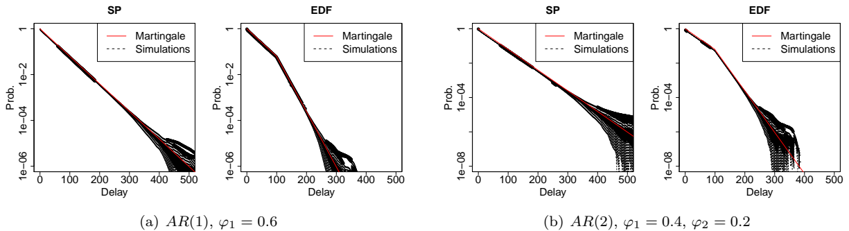
Figure 5: CCDF of the packet delay for AR(1) ((a)) and AR(2) ((b)), with parameters \mu = 0.5 , \sigma = 1 , utilization \rho = 0.95 , and, for EDF, y = d - d' = 99 .
