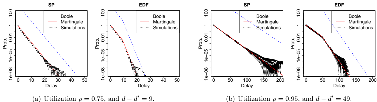
Figure 3: CCDF of the packet delay with N_1 = \frac{1}{2}N = 10 , \alpha = 0.1 , \beta = 0.5 , and R = 1 .
