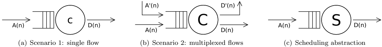
Figure 1: Two scenarios: (a) consists of a single flow A , whereas (b) has an additional cross-flow A' , in (c) the cross-flow from (b) is encoded in the dynamic service process S .
